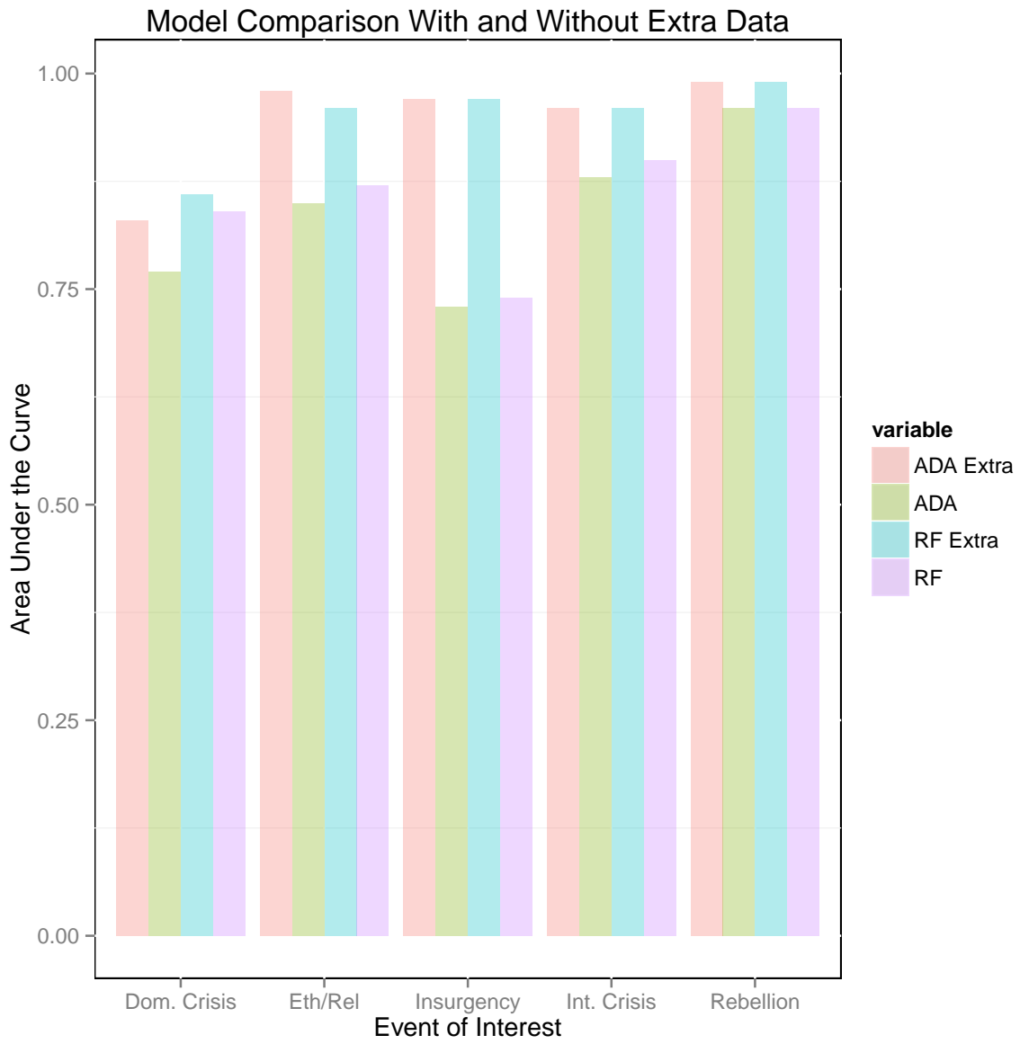
Figure 40: Impact of External Data
