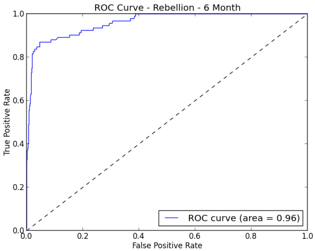
Figure 31: Rebellion Results
