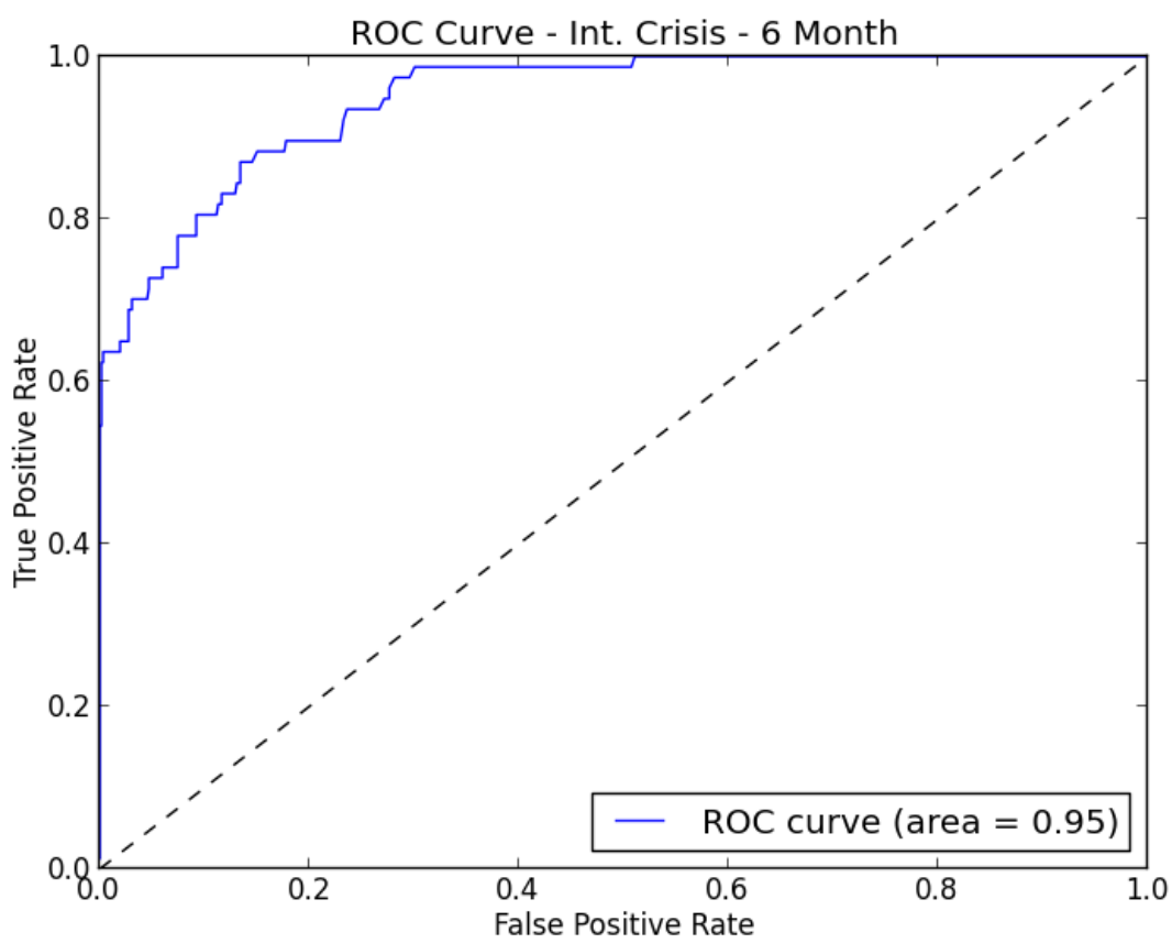
Figure 30: International Crisis Results
