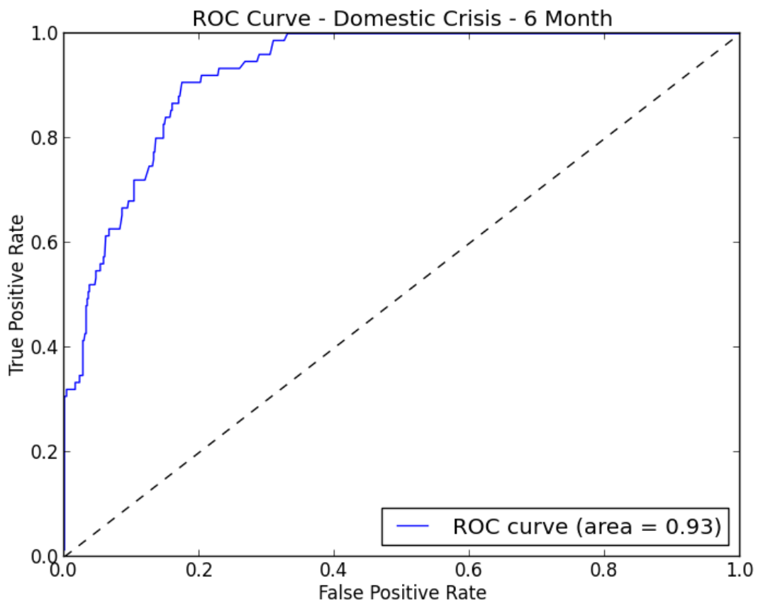
Figure 27: Domestic Crisis Results
