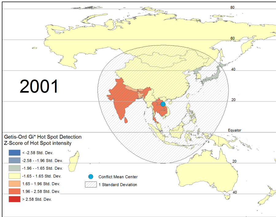
Figure 14: Hot/cold spots of gov_gov_matchf variable ratio
