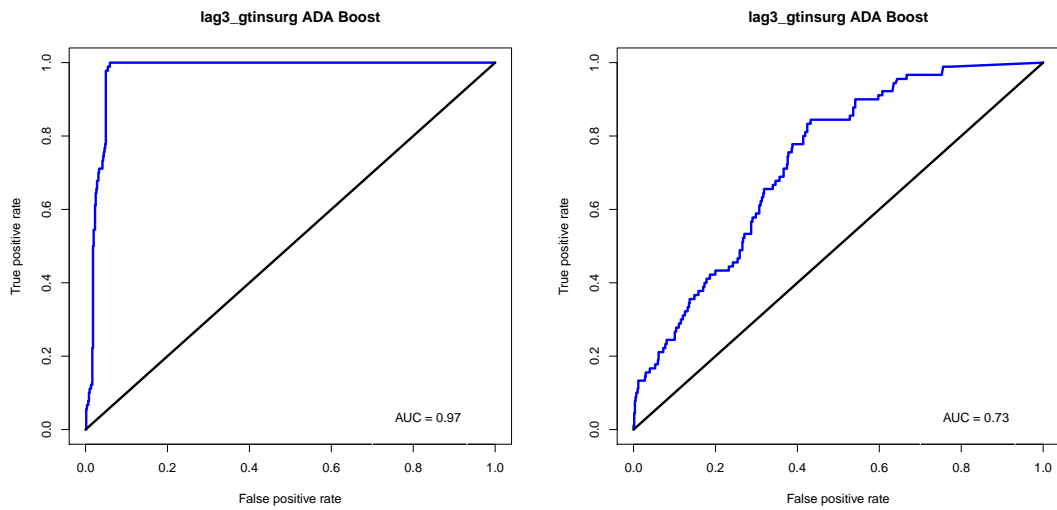
Figure 39: Insurgency EOI with Additional Variables
