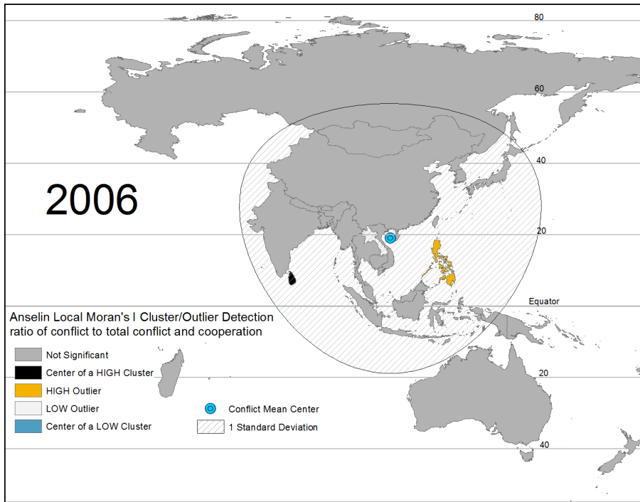
Figure 12: Clusters/outliers of gov_gov_matchf variable ratio
