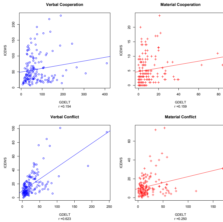
Figure 4: Comparison of ICEWS and GDELT Quadcounts: India→Pakistan 1998-2010
