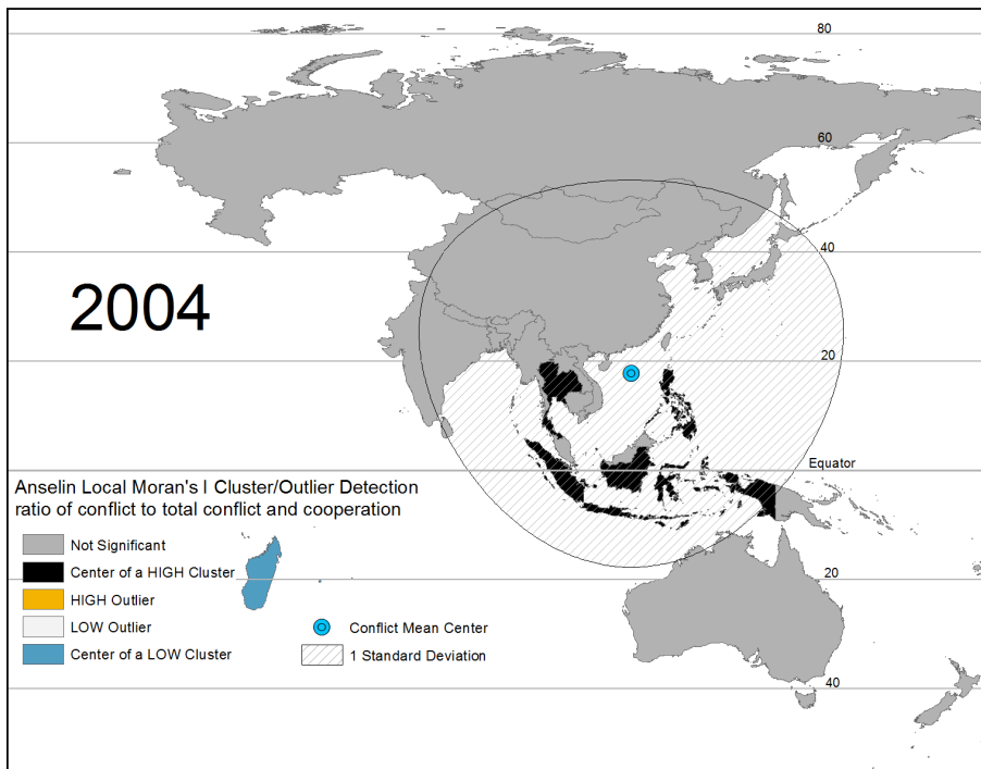
Figure 11: Clusters/outliers of gov_gov_matchf variable ratio
