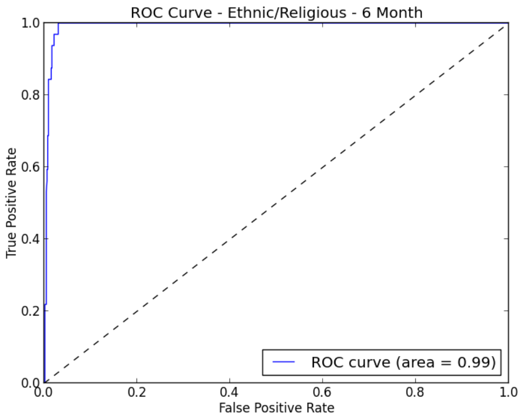
Figure 28: Ethnic/Religious Results
