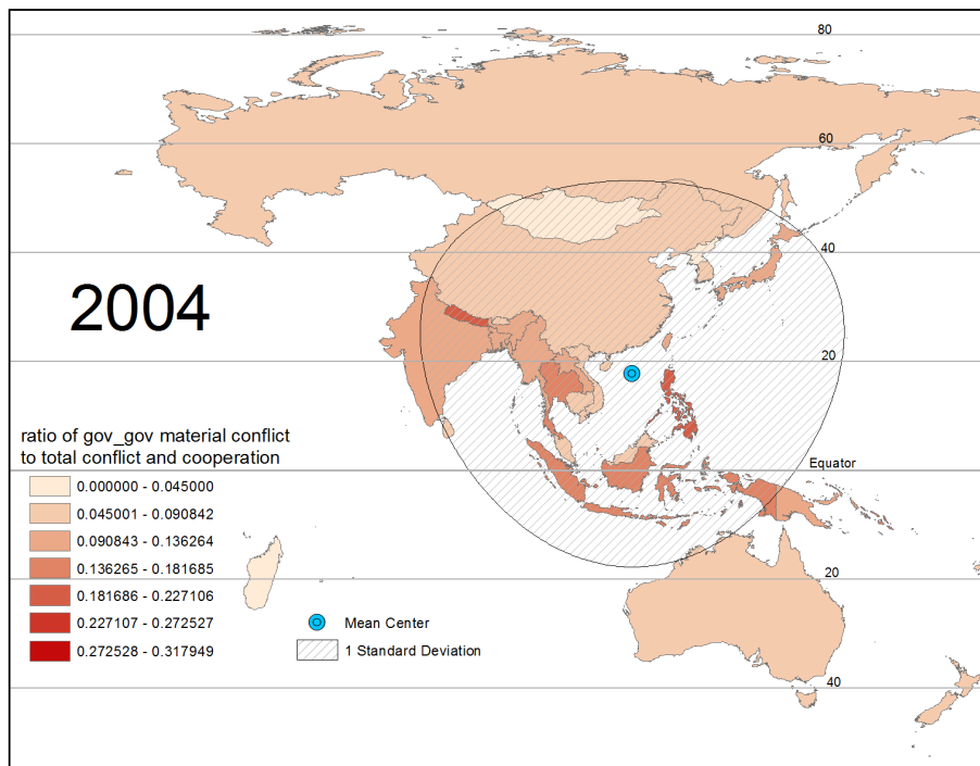
Figure 8: gov_gov_matchf as a ratio to total material and verbal cooperation and conflict.
