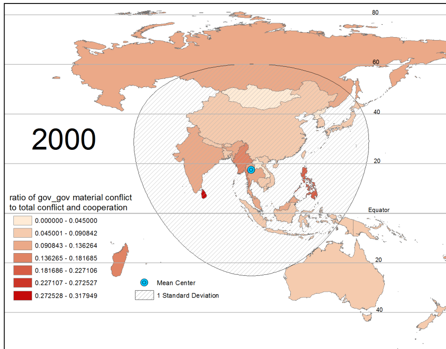
Figure 7: gov_gov_matchf as a ratio to total material and verbal cooperation and conflict.
