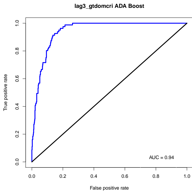
Figure 34: Domestic Crisis
