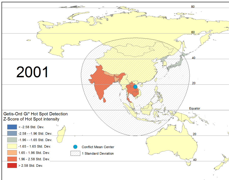
Figure 15: Hot/cold spots of gov_gov_matchf variable ratio
