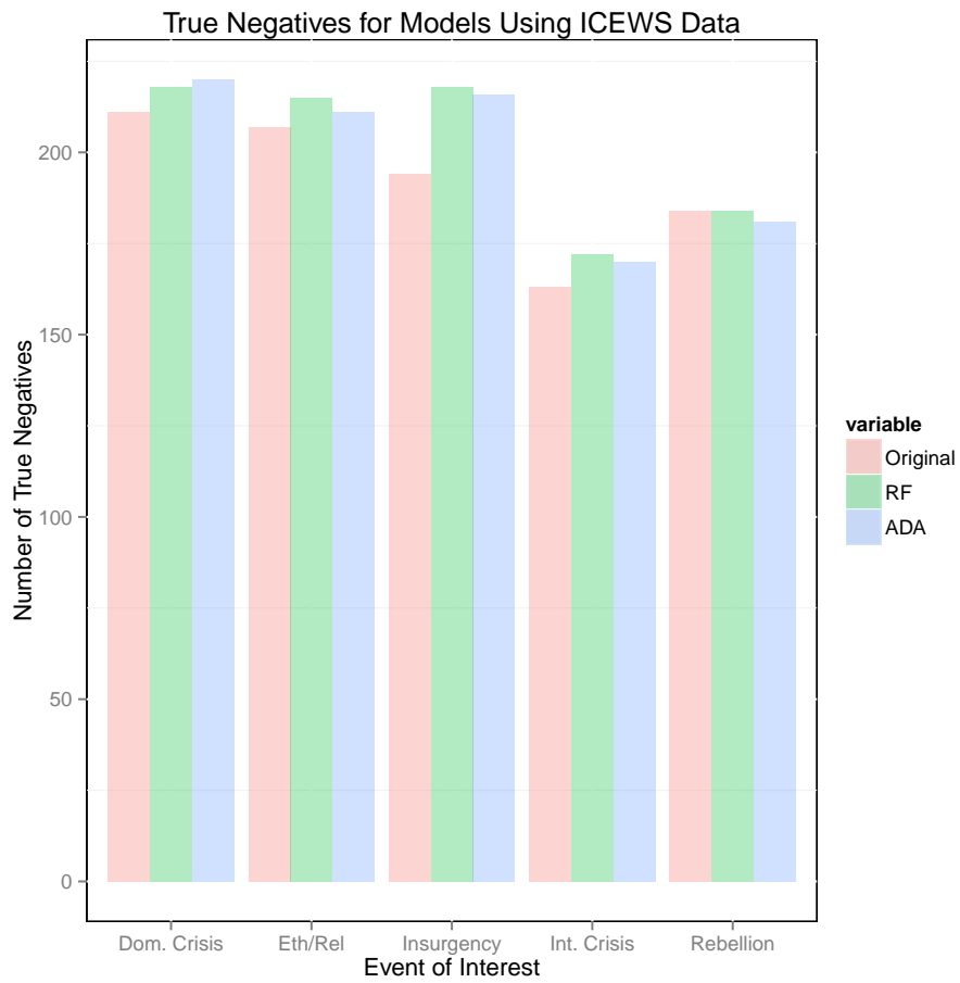
Figure 26: True Negative Comparison
