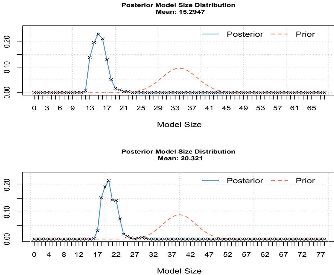
Figure 19: Posterior Model Size Distributions for Events Model and Full Model (International Crisis)
