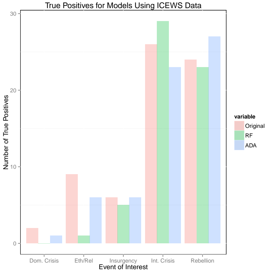
Figure 25: True Positive Comparison
