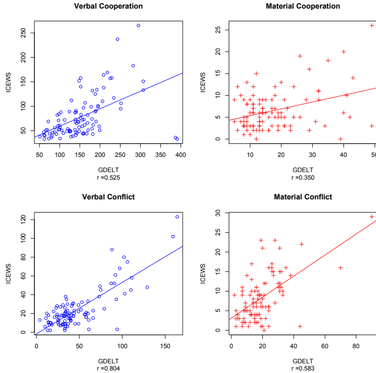
Figure 3: Comparison of ICEWS and GDELT Quadcounts: China→Taiwan 1998-2010 with VERCP < 30 cases removed
