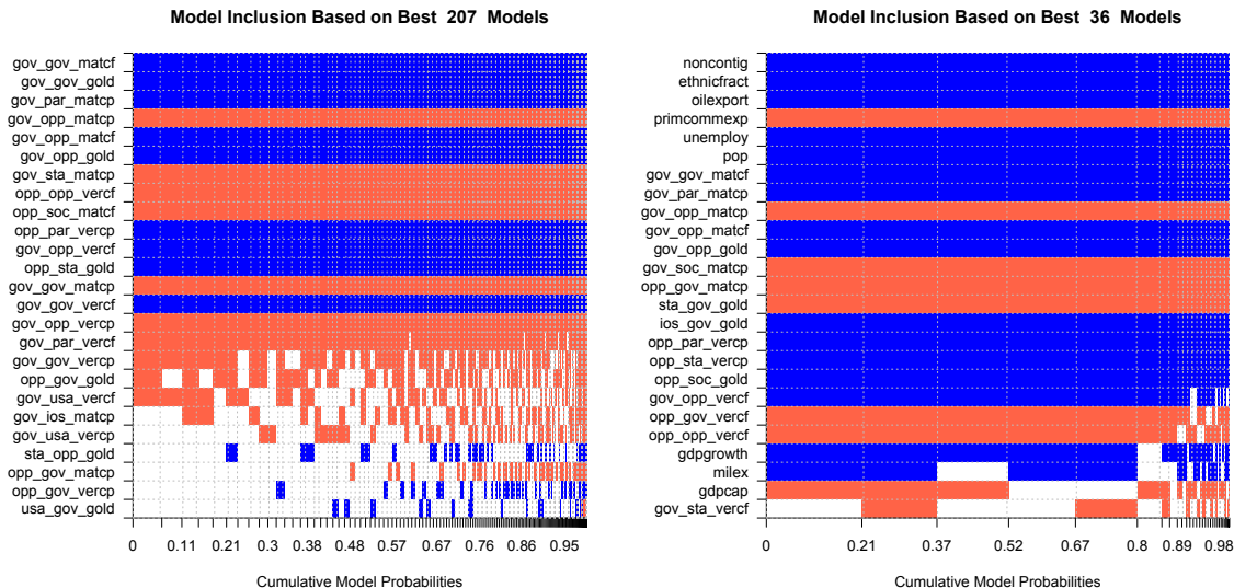
Figure 16: Variable Inclusion for Events Model and Full Model (Rebellion)
