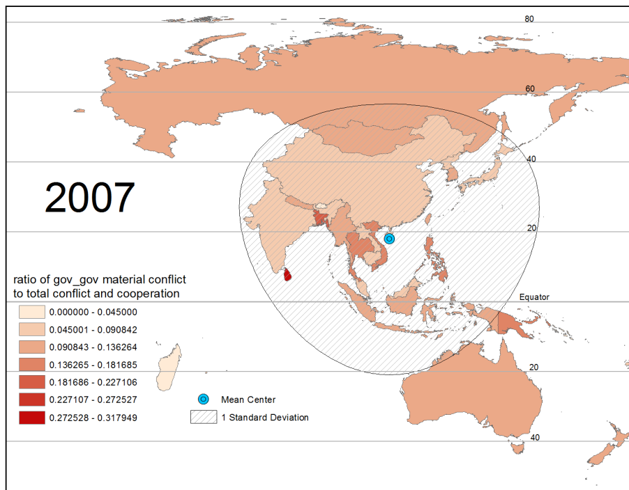
Figure 9: gov_gov_matcf as a ratio to total material and verbal cooperation and conflict.
