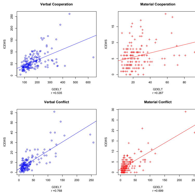
Figure 5: Comparison of ICEWS and GDELT Quadcounts: South Korea→North Korea 1998-2010
