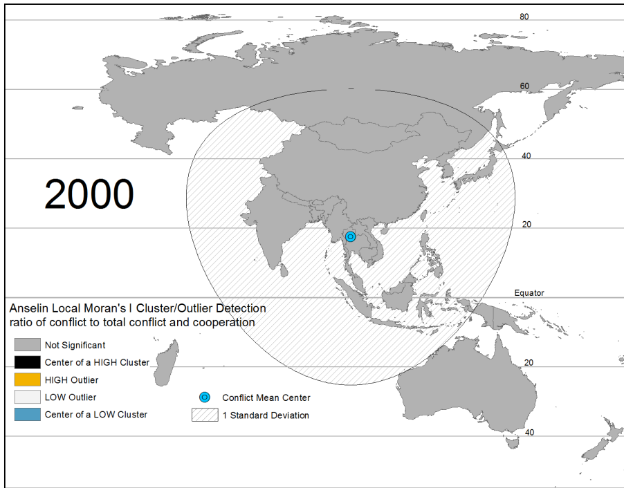
Figure 10: Clusters/outliers of gov_gov_matchf variable ratio
