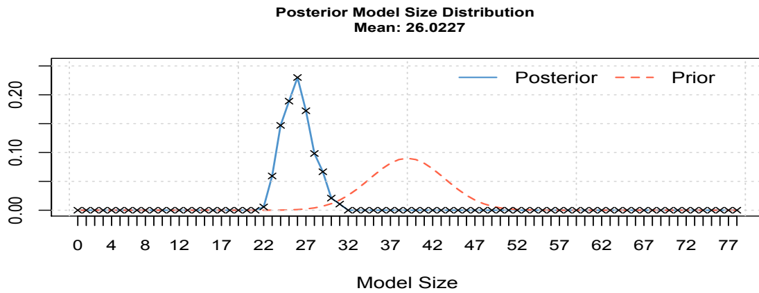
Figure 17: Posterior Model Size Distributions for Events Model and Full Model (Rebellion)
