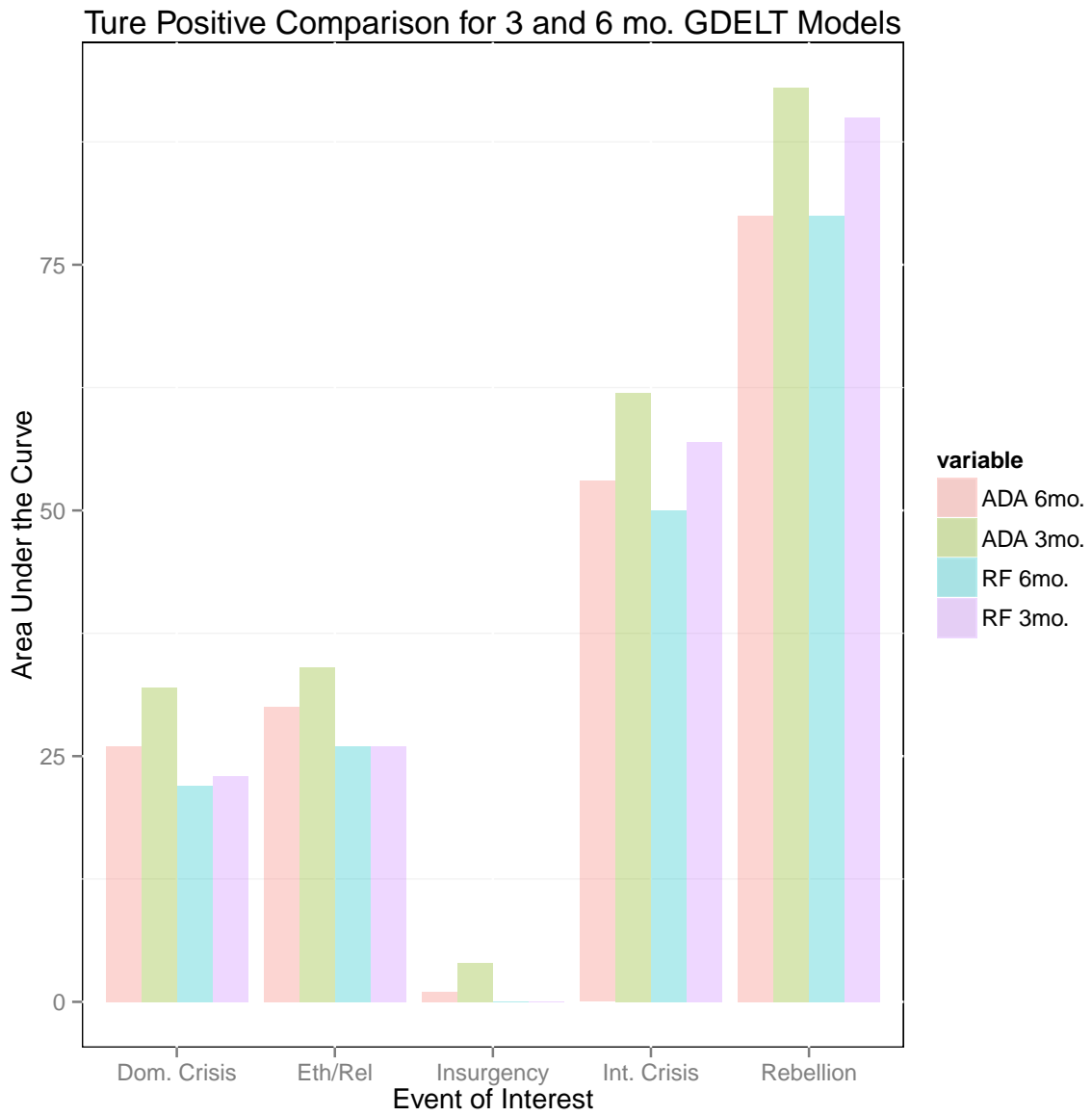
Figure 37: True Positives
