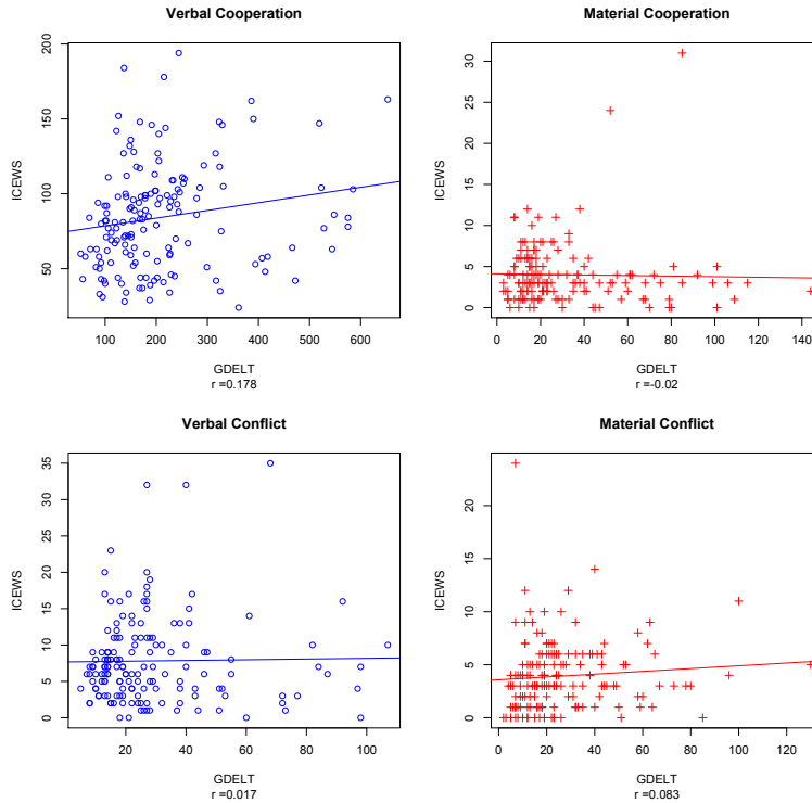
Figure 6: Comparison of ICEWS and GDELT Quadcounts: USA→Japan 1998-2010
