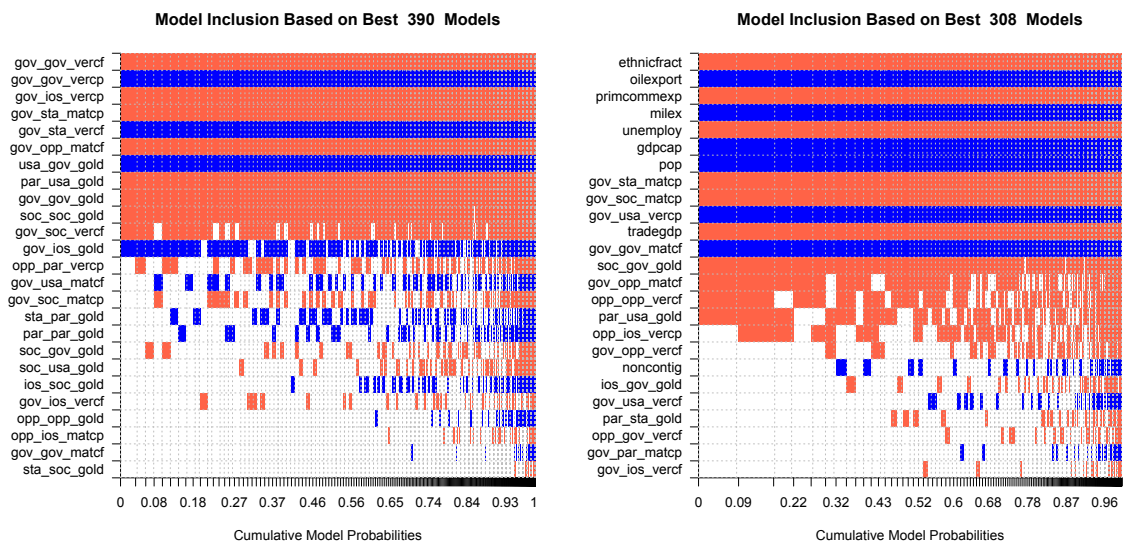
Figure 18: Variable Inclusion for Events Model and Full Model (International Crisis)
