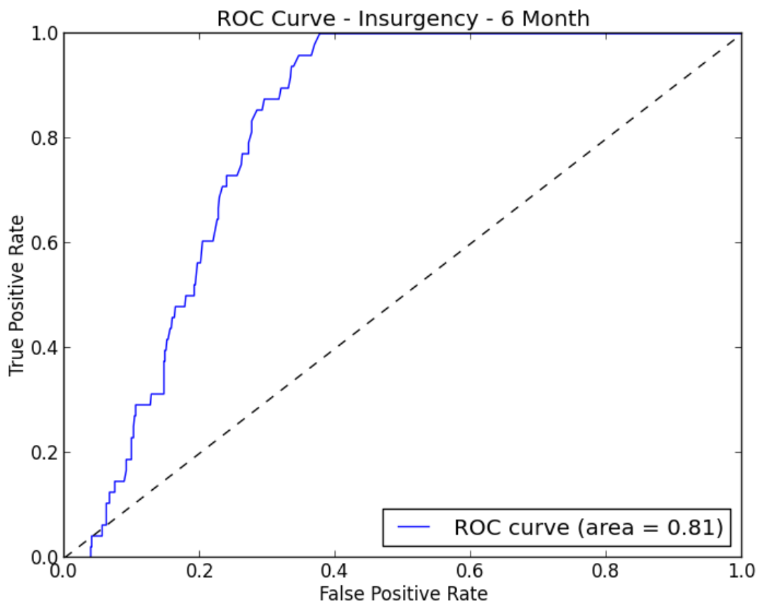
Figure 29: Insurgency Results
