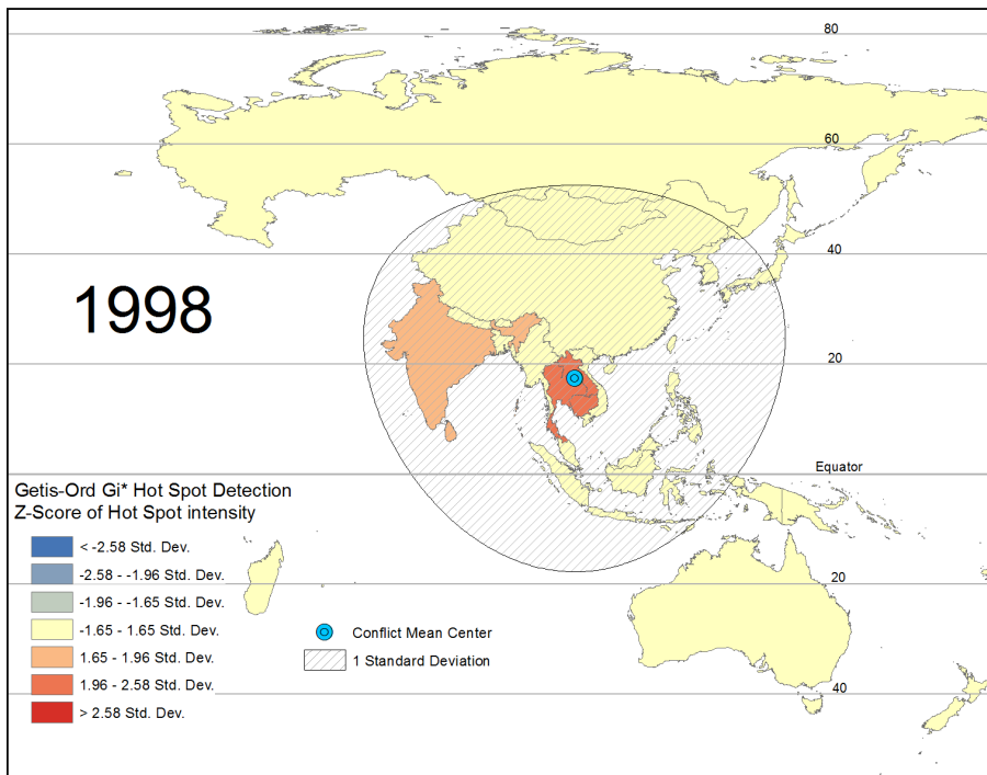
Figure 13: Hot/cold spots of gov_gov_matchf variable ratio
