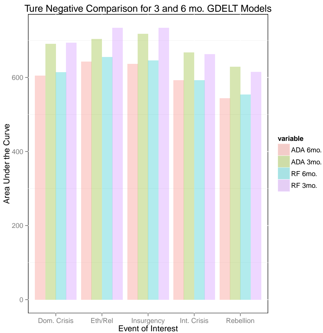
Figure 38: True Negatives
