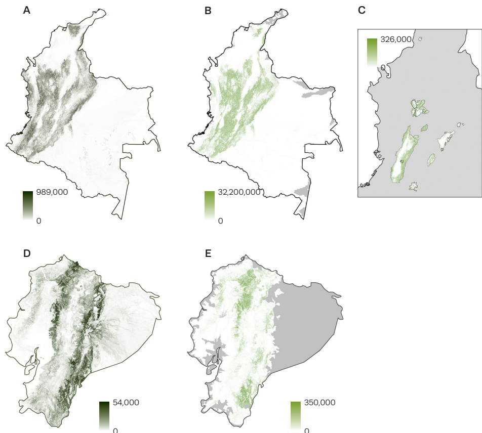
FIGURE 4 Erosion regulation for drinking water quality and reservoir maintenance in 2000.
