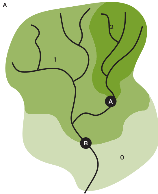
FIGURE 1 Hypothetical depiction of servicesheds for water-related regulating services. In watershed Area “0”
