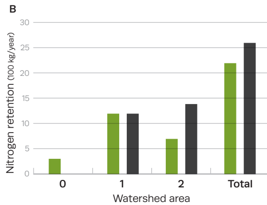
FIGURE 1 Hypothetical depiction of servicesheds for water-related regulating services. In watershed Area “0”
